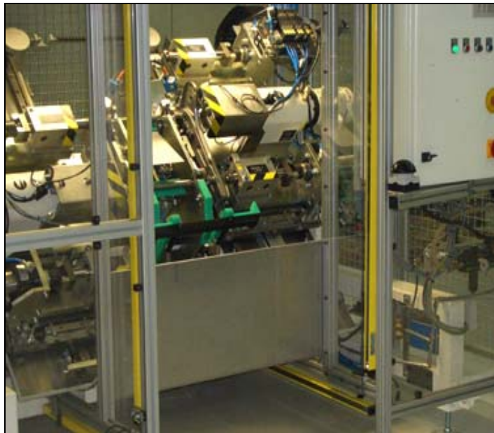
The tube forming machine at Faurecia with the yellow Safe4 emitter and receiver light curtains
